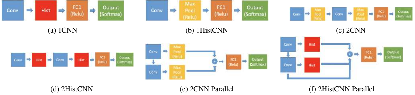
Figure 1: Architectures used for each texture dataset.
