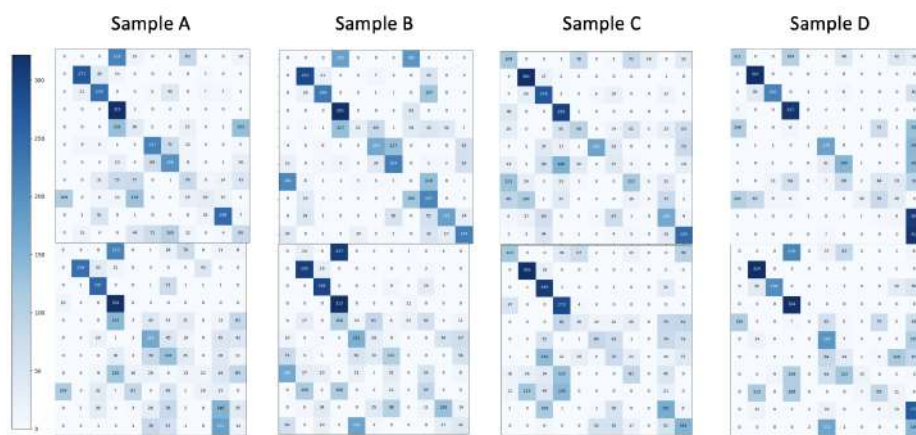
Figure 12: Confusion Matrices for 2_CNN_parallel (top row) and 2_HistCNN_parallel (bottom row)
