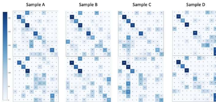
Figure 10: Confusion Matrices for 1_CNN (top row) and 1_HistCNN (bottom row)
